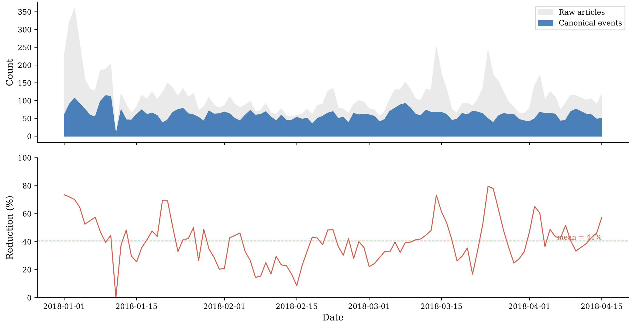
Daily Article Volume and Clustering Reduction
